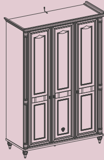
3 DOORS WARDROBE W: 140x H: 203 x D: 58 cm 20.21.1002.03
